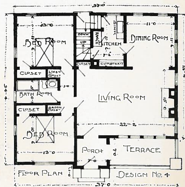
PLAN No. 4
