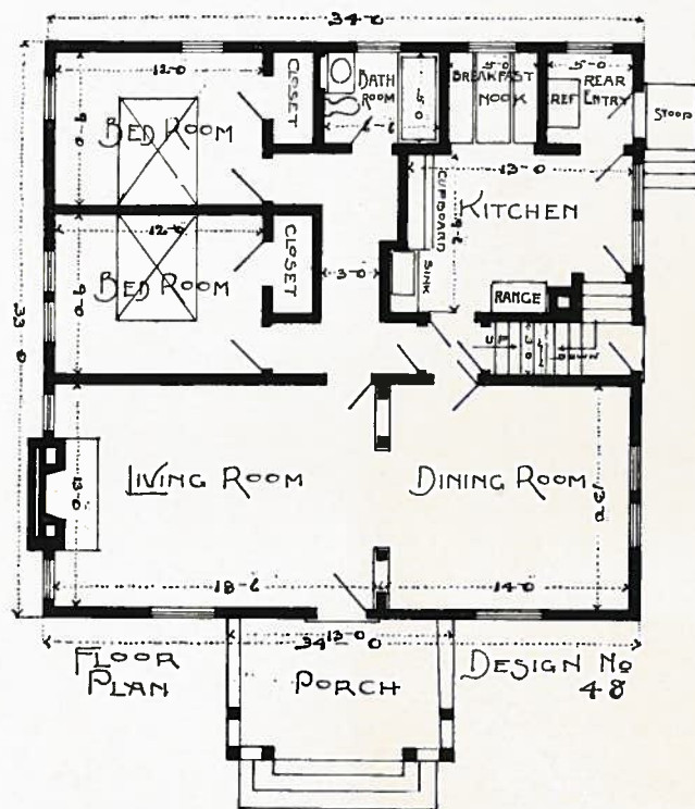
PLAN No. 48
