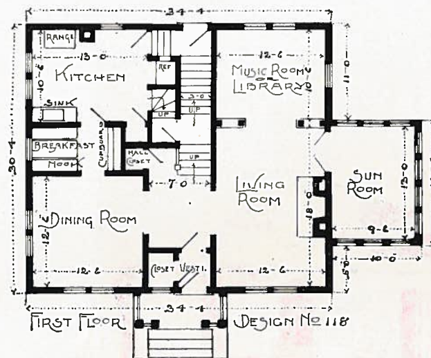
PLAN No. 118
