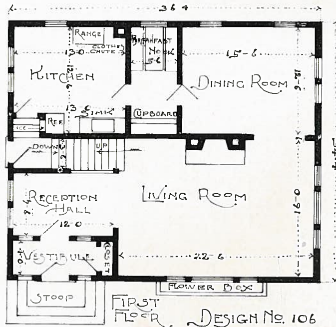
PLAN No. 106
