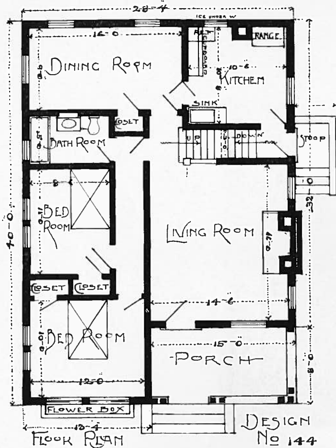
PLAN No. 144
