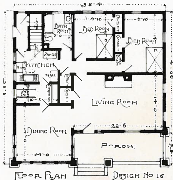
PLAN No. 16
