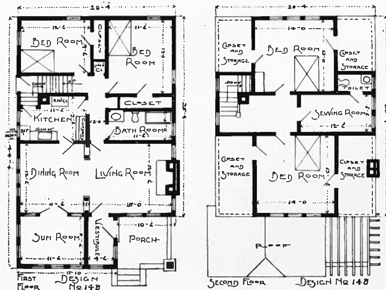
PLAN No. 148
