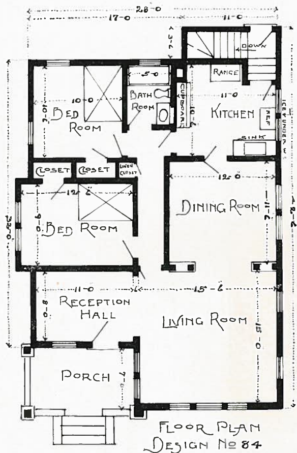
PLAN No. 84
