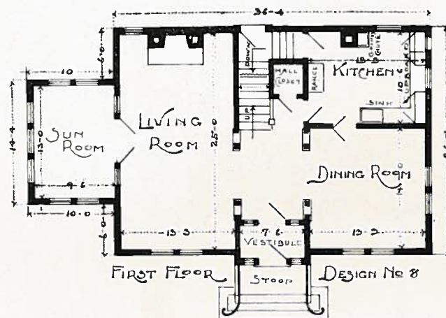
PLAN No. 8
