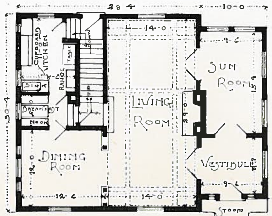
FIRST FLOOR DESIGN No. 52
