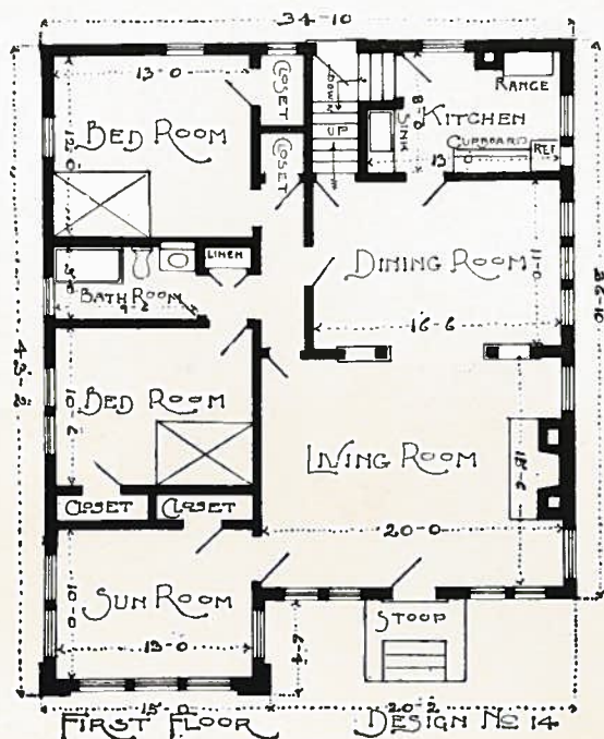
PLAN No. 14
