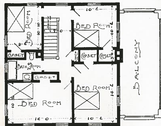
SECOND FLOOR DESIGN No. 52
