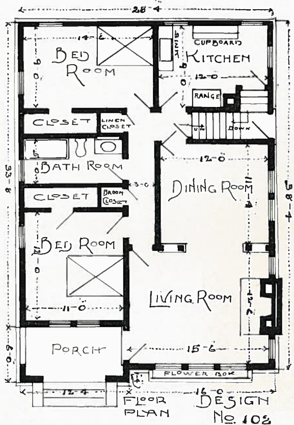
PLAN No. 102
