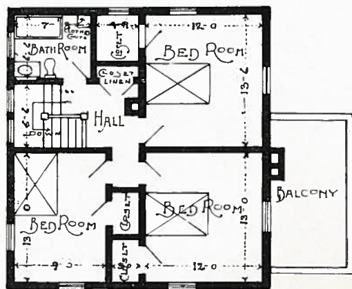
SECOND FLOOR DESIGN No. 52A
