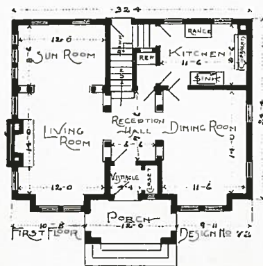
PLAN No. 72
