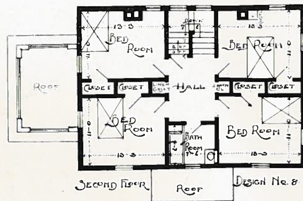
PLAN No. 8
