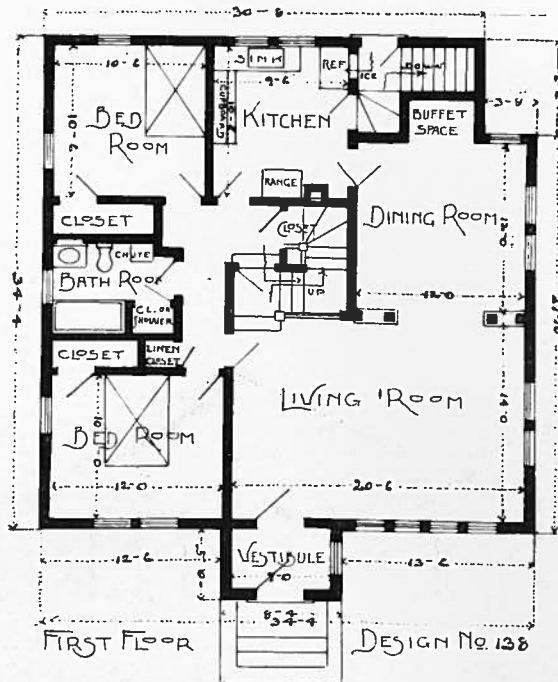
PLAN No. 138
