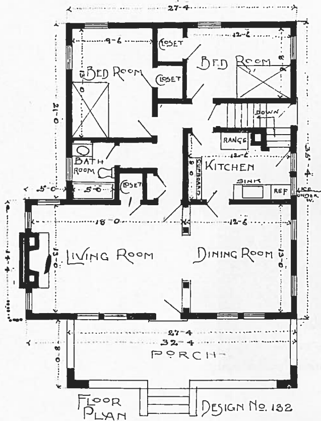
PLAN No. 132
