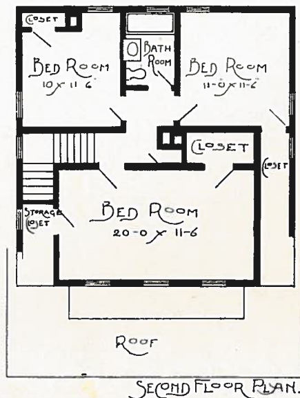
PLAN No. 94
