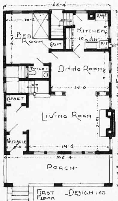
PLAN No. 162
