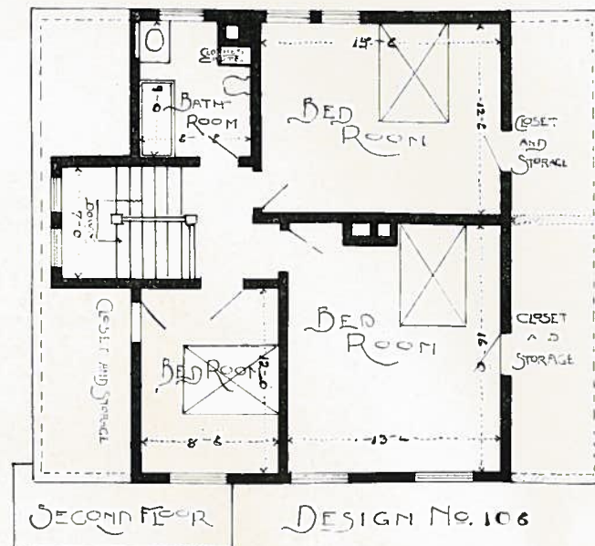
PLAN No. 106
