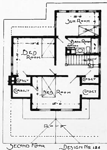
PLAN No. 126
