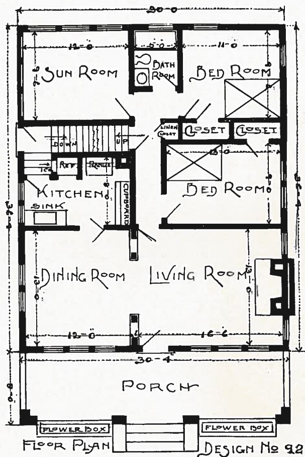
PLAN No. 92
