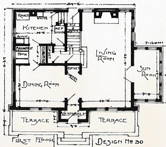
PLAN No. 30
