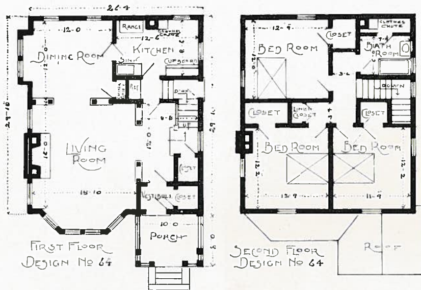
PLAN No. 64
