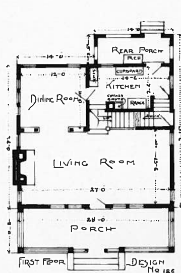
PLAN No. 126
