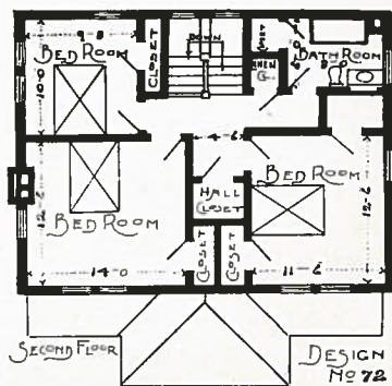
PLAN No. 72
