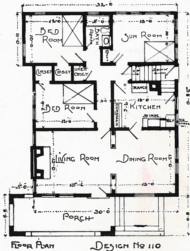
PLAN No. 110
